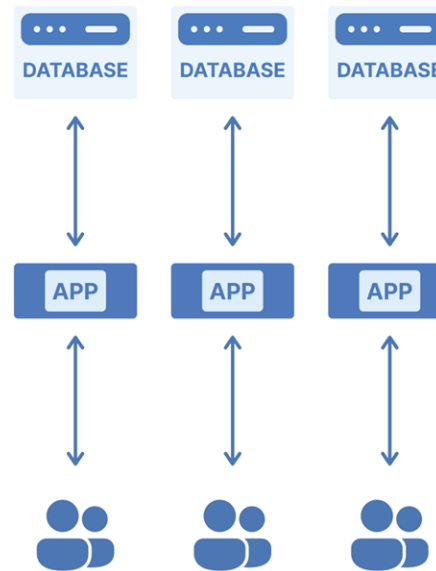
SINGLE TENANT (MULTI - INSTANCES) ONE CLIENT PER APPLICATION INSTANCE - CLIENTS DO NOT SHARE APPLICATION OR THE DATABASE
